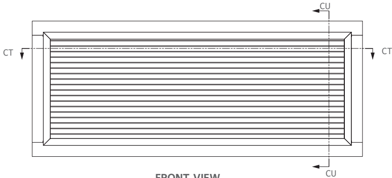
FRONT VIEW WITH WALL SLEEVE / PTAC UNIT N.T.S.
