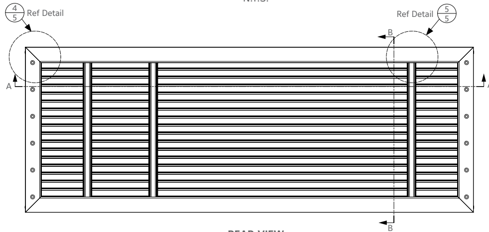
REAR VIEW AEL- 42 - 7020 WINDLOAD - 50 PSF
