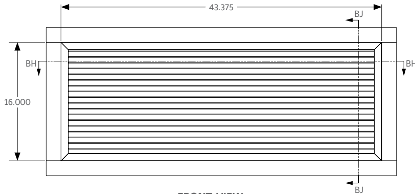
FRONT VIEW WITHOUT WALL SLEEVE / PTAC UNIT N.T.S.
