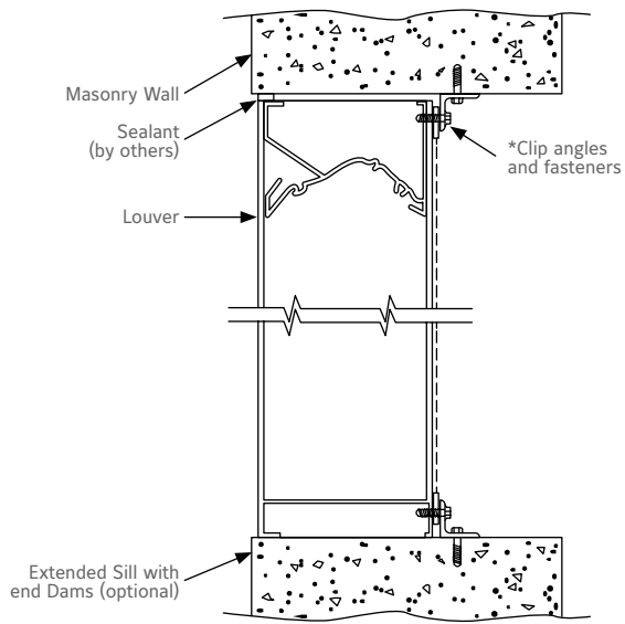
MASONRY WALL
