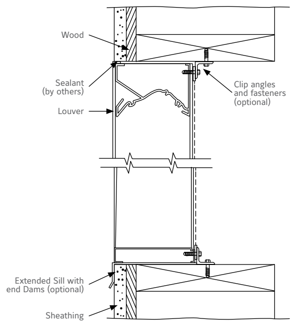
WOOD INSTALLATION
