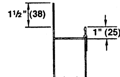
Integral Flange
