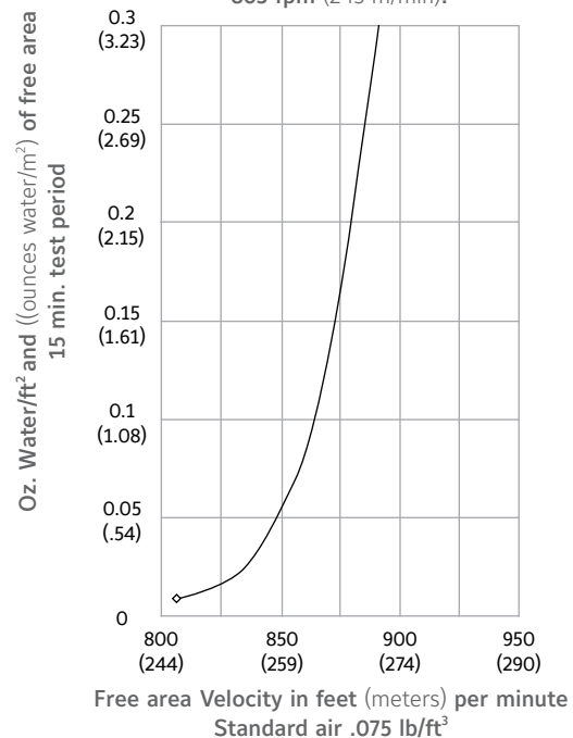
Water Penetration Graph Test size 48" wide X 48" high (1219 X 1219) Beginning point of water penetration at .01 oz. /sq. ft. is 803 fpm (245 m/min).
