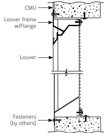
FLANGE MOUNT
