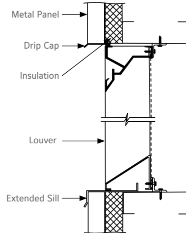
METAL PANEL WALL
