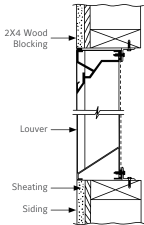
WOOD INSTALLATION
