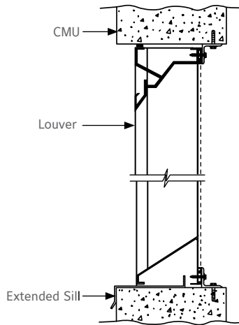
MASONRY WALL
