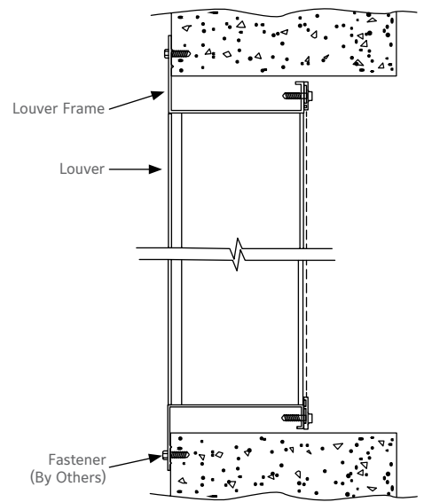
FLANGE MOUNT
