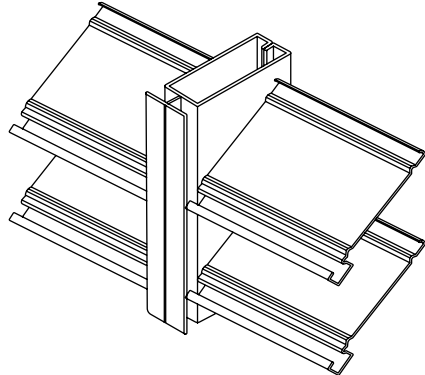
Visible Mullion At Section Joints
